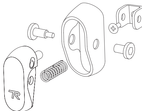
Art. No. LS319. Set Right + Left.
