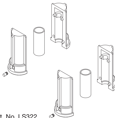
Art. No. LS322. Set Right + Left.
